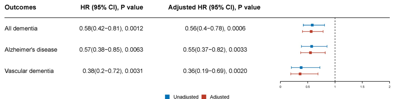
Fig 3. HRs, 95% CIs, and p -values for the association of lithium with the development of dementia (and its subtypes) by Cox proportional hazards models. HRs, 95% CIs, and p -values were extracted from inverse probability weighted Cox regression. Adjusted HRs were adjusted for age, sex, marital status, ethnicity, smoking status, alcohol disorders, antipsychotic use, depression, mania or BPAD, hypertension, central vascular disease, diabetes mellitus, and hyperlipidemias. The AIC was 14,275 for the model fitted for all dementias, 13,240 for the model fitted for AD, and 13,220 for the model fitted for VD. AD, Alzheimer's disease; AIC, Akaike information criterion; BPAD, bipolar affective disorder/mania; CI, confidence interval; HR, hazard ratio; VD, vascular dementia.
