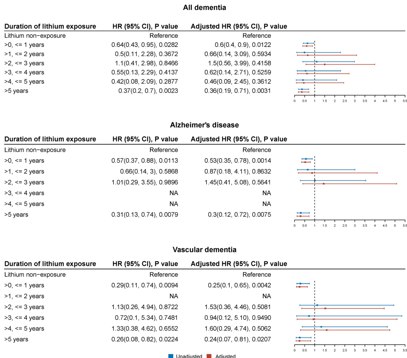
Fig 4. HRs, 95% CIs, and p -values for the association of duration of lithium exposure with the development of dementia (and its subtypes) by Cox proportional hazards models. HRs, 95% CIs, and p -values were extracted from inverse probability weighted Cox regression. Adjusted HRs were adjusted for age, sex, marital status, ethnicity, smoking status, alcohol disorders, antipsychotic use, depression, mania or BPAD, hypertension, central vascular disease, diabetes mellitus, and hyperlipidemia. NA indicates no result (no corresponding cases). The AIC was 14,125 for the model fitted for all dementias, 13,064 for the model fitted for AD, and 13,119 for the model fitted for VD. See Fig Q in S1 Appendix for an equivalent analysis using pooled intermediate durations and Fig R in S1 Appendix for the effects of lithium exposure duration as a continuous variable. AD, Alzheimer disease; AIC, Akaike information criterion; BPAD, bipolar affective disorder/mania; CI, confidence interval; HR, hazard ratio; VD, vascular dementia.
