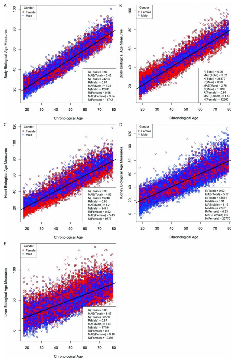
Figure 2. Correlations between chronological age and calculated biological ages. Each panel displays a scatter plot of chronological age (x-axis) versus a specific biological age (y-axis) for the entire dataset. The solid black line in each panel represents the linear regression line of best fit. (A) Body biological age calculated using the newly developed 13-biomarker model. (B) Body biological age calculated using the original features from Levine et al. [41]. (C) Heart biological age. (D) Kidney biological age. (E) Liver biological age. The specific biomarkers used for each model are detailed in Supplementary Table 1. Abbreviations: R, Pearson correlation coefficient; MAE, mean absolute error in years; N, sample size.
