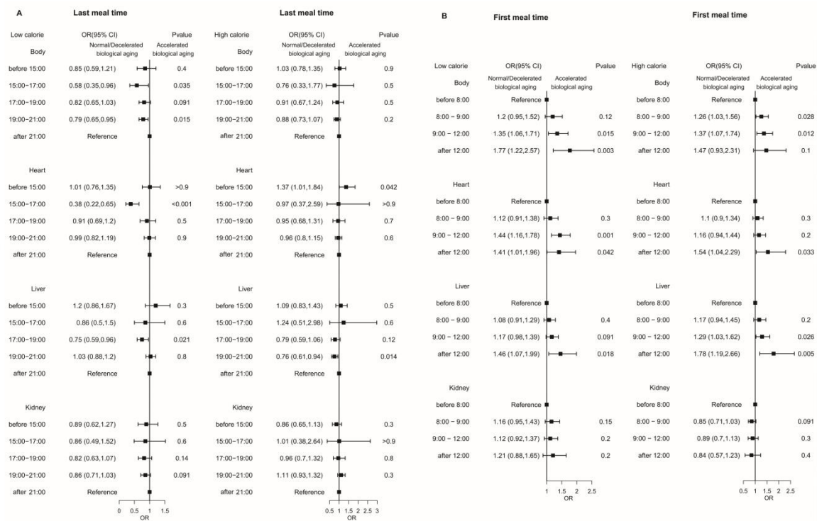
Figure 4. Association of last meal time (A) and first meal time (B) with the biological aging risk of the body and organs by caloric intake. Number = 14012. OR indicates odds ratio. CI indicates confidence interval; Ref indicates reference. The multivariate logistic regression models adjusted for feeding duration (continuous), age (continuous), gender (male or female), race (non-Hispanic White, non-Hispanic Black, Mexican American, or other Race), poverty ratio (continuous), education level (below high school, high school or above high school), drinking status (non-drinker or <1 drinks/month, 1-5 drinks/month, 5-10 drinks/month or 10+ drinks/month), smoking status (never smoker, former smoker or current smoker), body mass index (underweight (<18.5), normal (18.5 to <25), overweight (25 to <30) or obese (30 or greater)), self-reported chronic obstructive pulmonary disease (yes or no), self-reported liver disease (yes or no), self-reported cancer (yes or no), self-reported cardiovascular disease (yes or no), self-reported hypertension (yes or no), self-reported diabetes (yes or no), self-reported kidney disease (yes or no), meal count (continuous), carbohydrate intake, fat intake, protein intake, and dietary fiber intake per kilogram of body weight (continuous).
