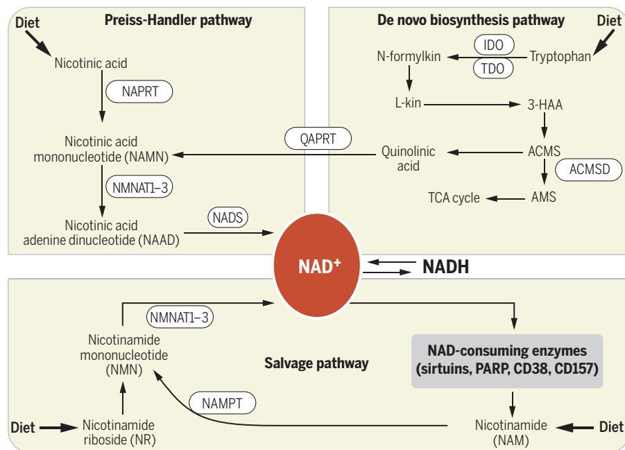
Fig. 2. NAD + biosynthetic pathways. NAD + levels are maintained by three independent pathways. First, the Preiss-Handler pathway uses dietary nicotinic acid and the enzyme nicotinic acid phosphoribosyltransferase (NAPRT) to generate NAMN, which is then transformed into NAAD by NAMN transferase (NMNAT). Three forms of this enzyme (NMNAT1, -2, and -3) have distinct subcellular localizations. The process is completed by the transformation of NAAD into NAD + by NAD + synthase (NADS). Second, the de novo synthesis pathway of NAD from tryptophan occurs through the kinurenine pathway (5). The first step in this pathway is the rate-limiting conversion of tryptophan to N -formylkinurenine ( N -formylkin) by either IDO or TDO. Formylkinurenine is transformed into L -kinurenine ( L -kin), 3-hydroxykinurenine, and 3-hydroxyanthranilic acid (3-HAA) and finally to ACMS. This compound can spontaneously condense and rearrange into quinolinic acid, which is transformed into NAMN, at which point it converges with the Preiss-Handler pathway. ACMS can also be decarboxylated into AMS by ACMS decarboxylase (ACMSD), leading to its oxidation into acetyl-CoA via the TCA cycle. Third, the NAD + salvage pathway recycles the nicotinamide generated as a by-product of the enzymatic activities of NAD + -consuming enzymes: sirtuins, PARPs, and the cADPR synthases (CD38 and CD157). Initially, NAMPT recycles nicotinamide into NMN, which is then converted into NAD + via the different NMNATs.
